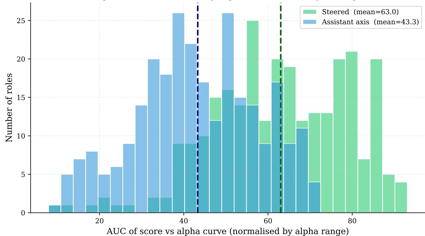
Score trajectory AUC distribution across 275 roles (higher AUC = consistently high scores across alpha range)
