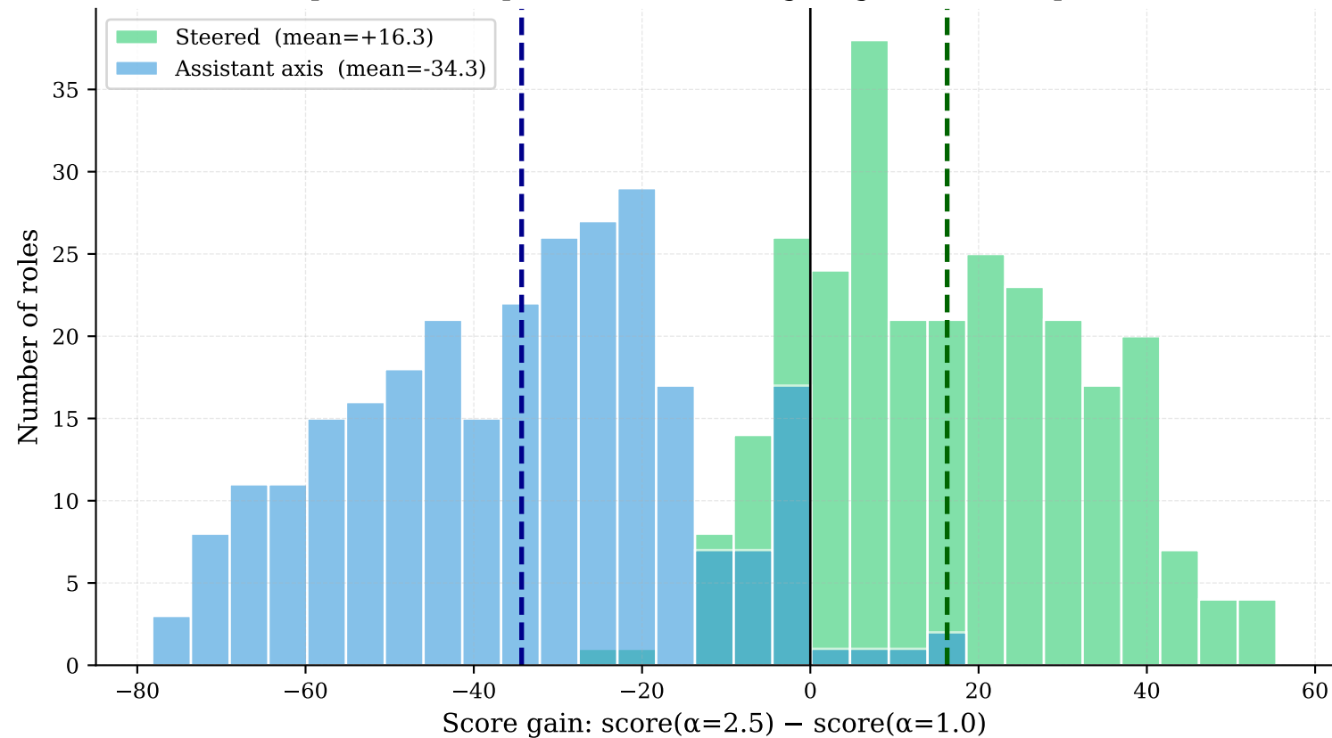
Score gain from low to high alpha: steered vs assistant axis (positive = improves with steering; negative = collapses)
