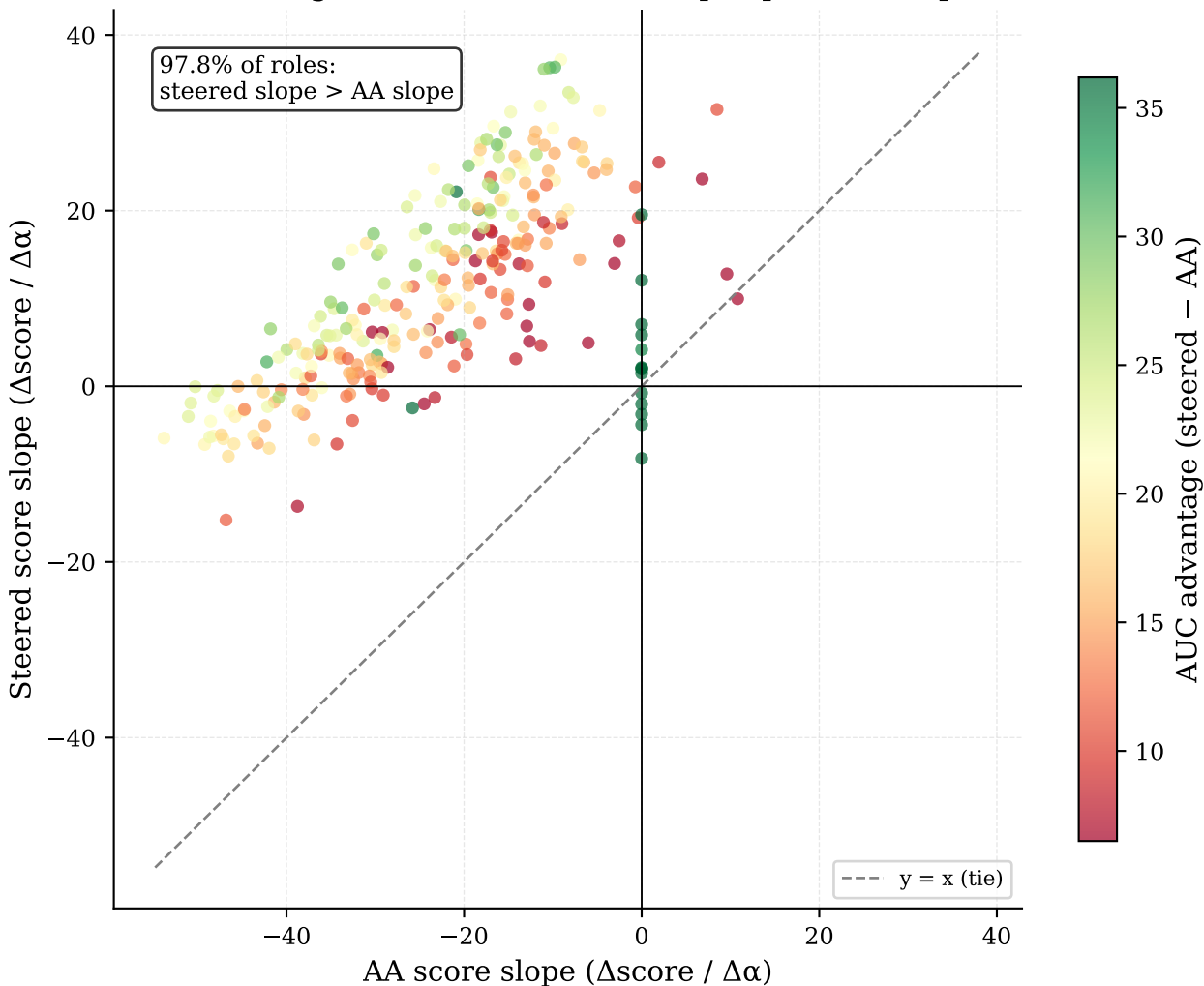
Per-role score slope: steered vs assistant axis (above diagonal = steered has steeper positive slope)
