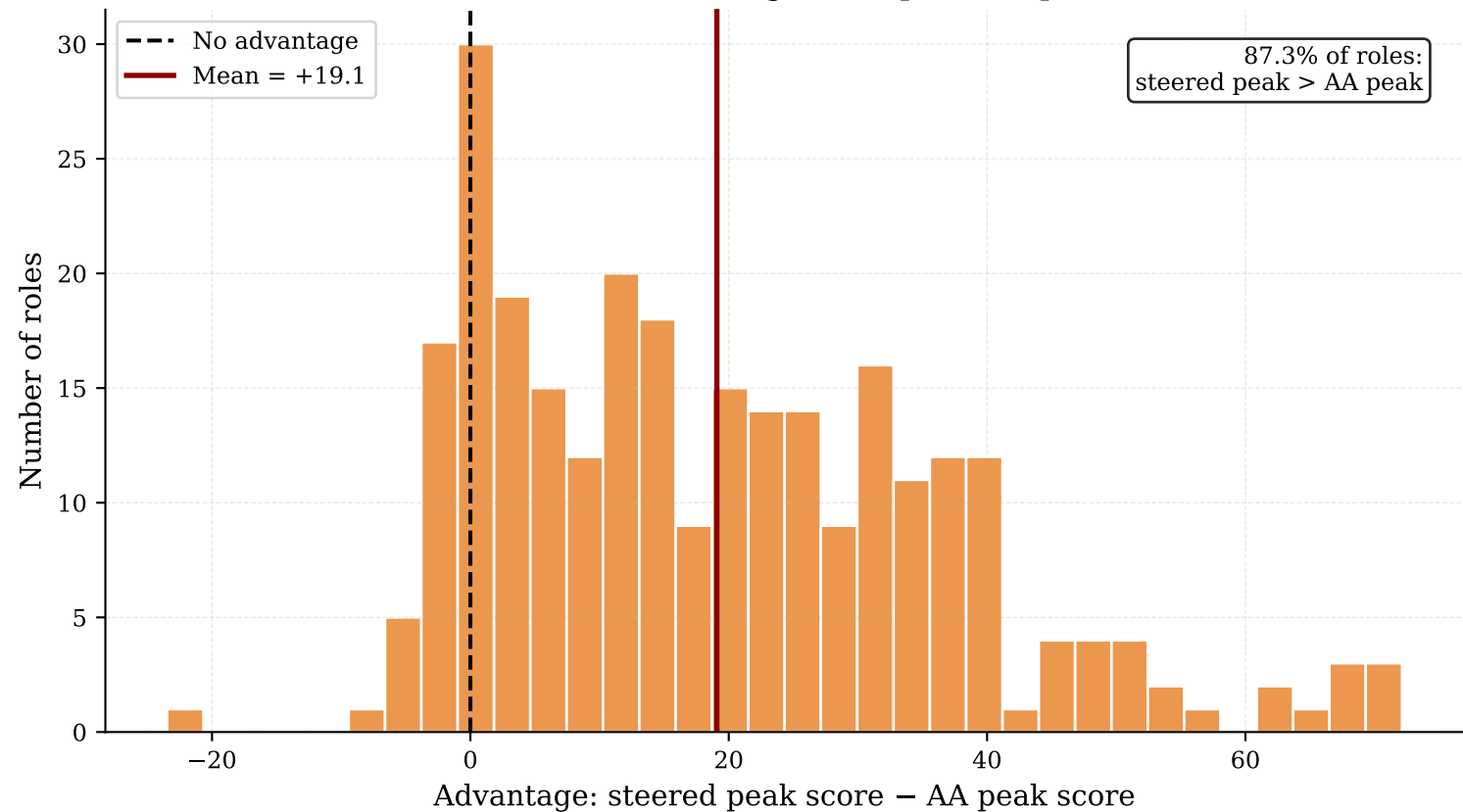
Distribution of best-vs-best advantage across 275 roles (both methods using their optimal alpha)
