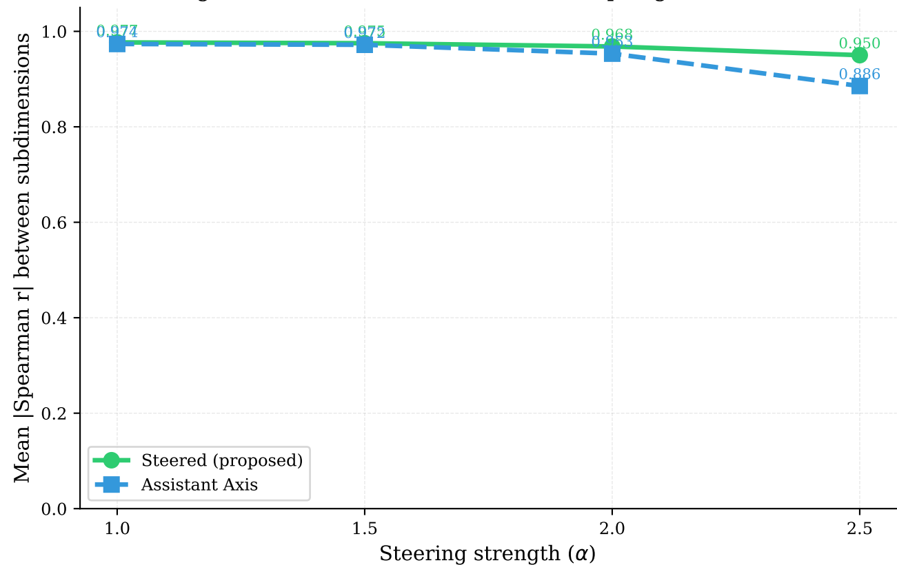
Subdimension inter-correlation vs steering strength (higher = behavioural dimensions collapsing toward one)
