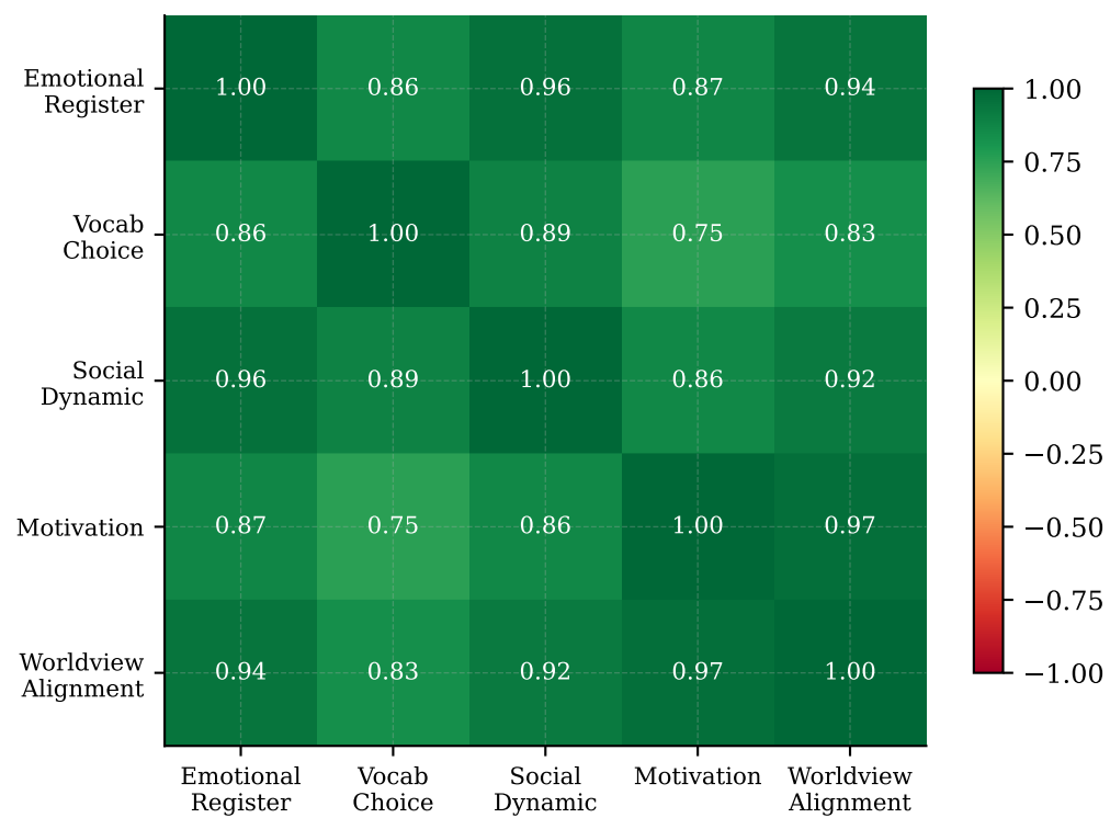
Assistant Axis — \alpha=2.5
