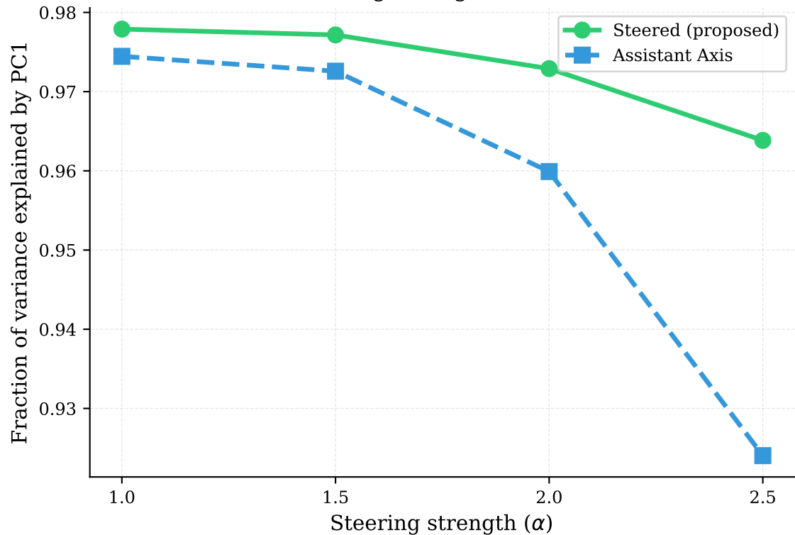
PC1 dominance (behavioural dimensionality) vs steering strength (275 roles)
