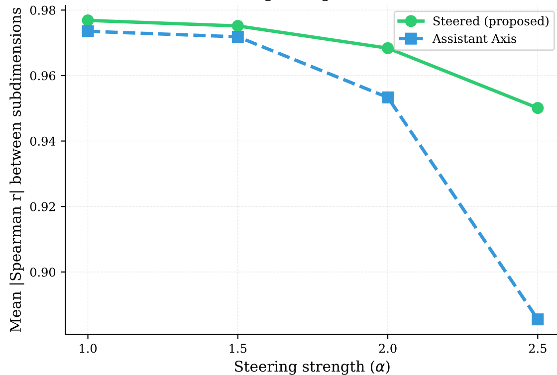
Inter-subdimension correlation vs steering strength (275 roles)
