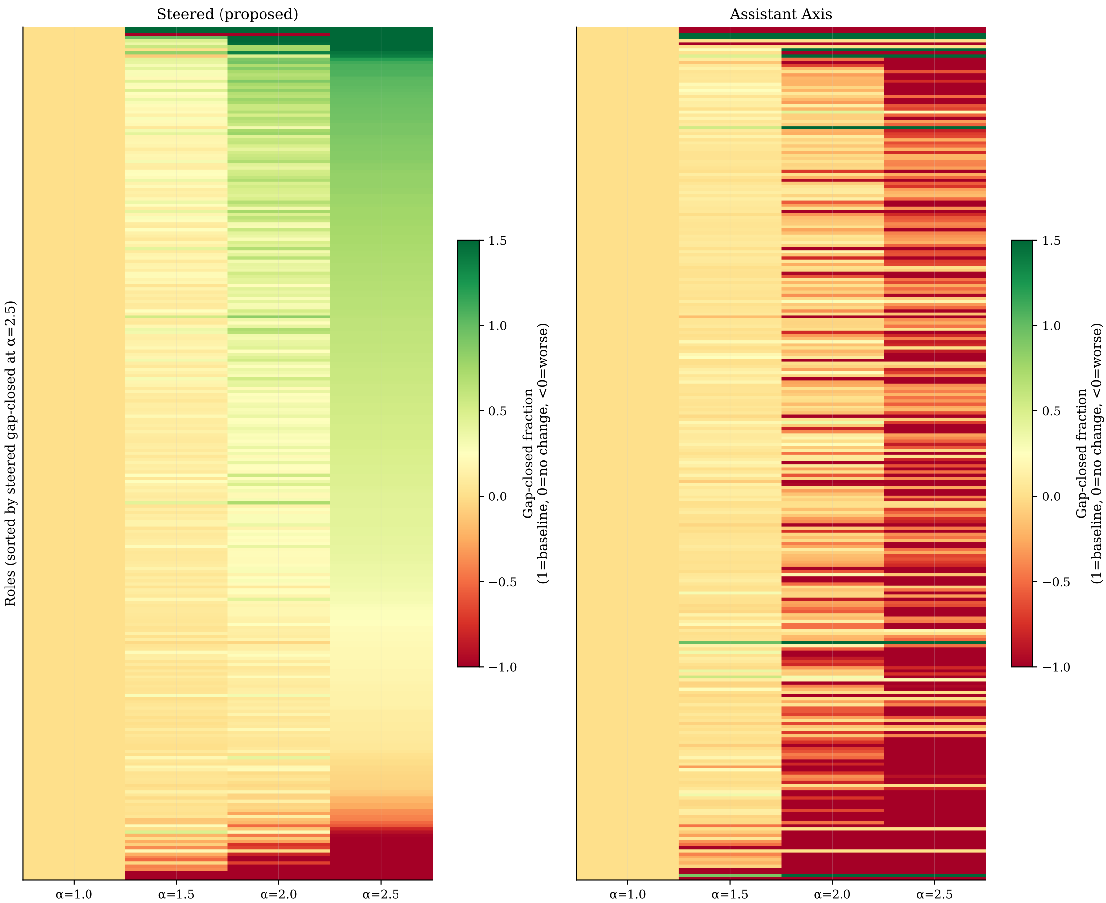
Per-role gap-closing fraction across all alphas
