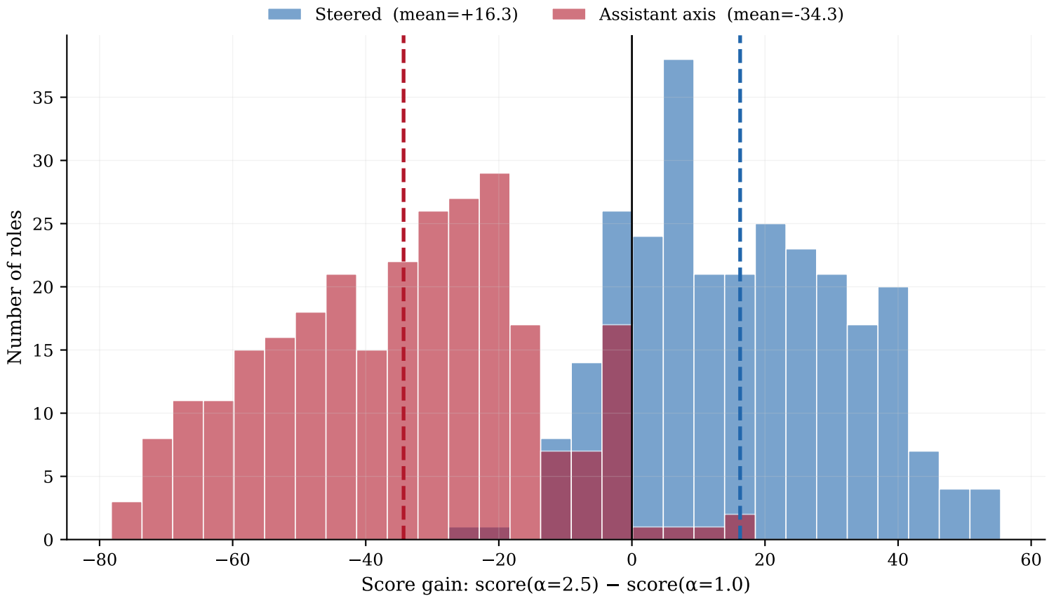
Score gain from low to high alpha: steered vs assistant axis
