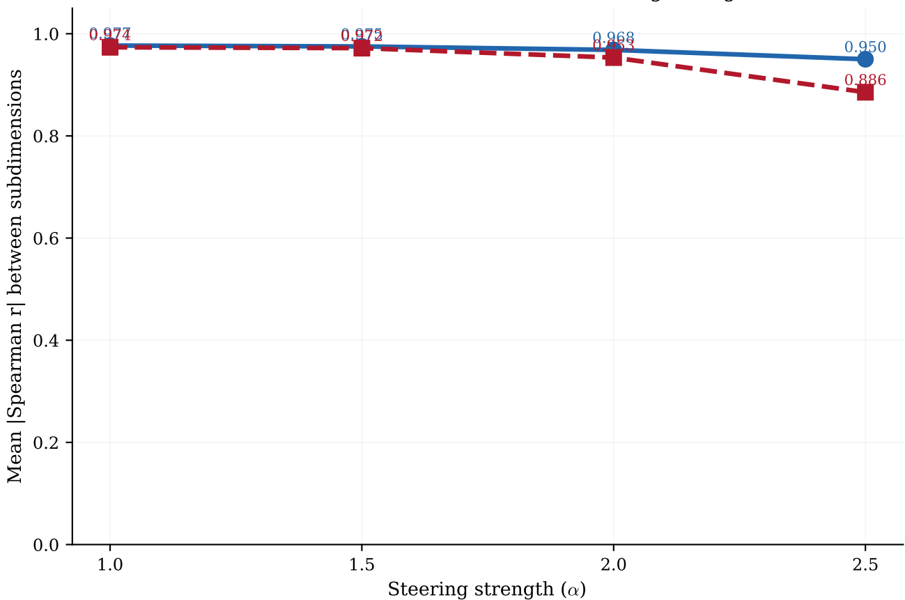
Subdimensionality inter-correlation vs steering strength
