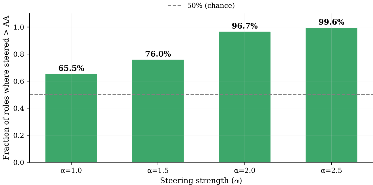
Win rate: fraction of 275 roles where steered beats AA
