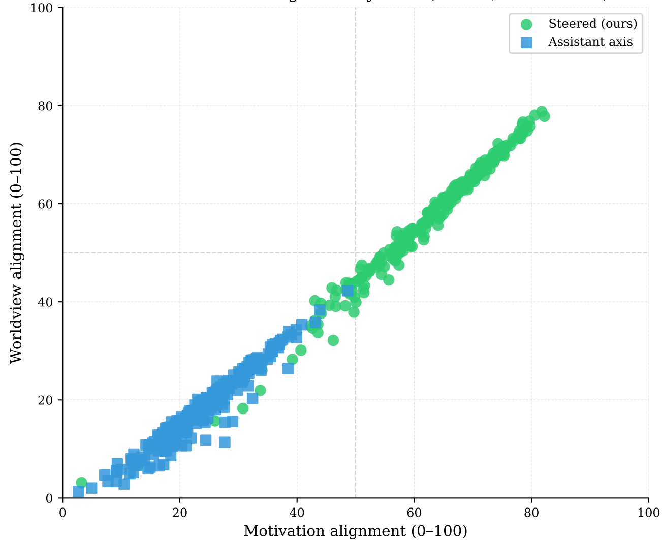
Content Dimension Alignment by Role ( \alpha = 2.5 , n=275 roles)
