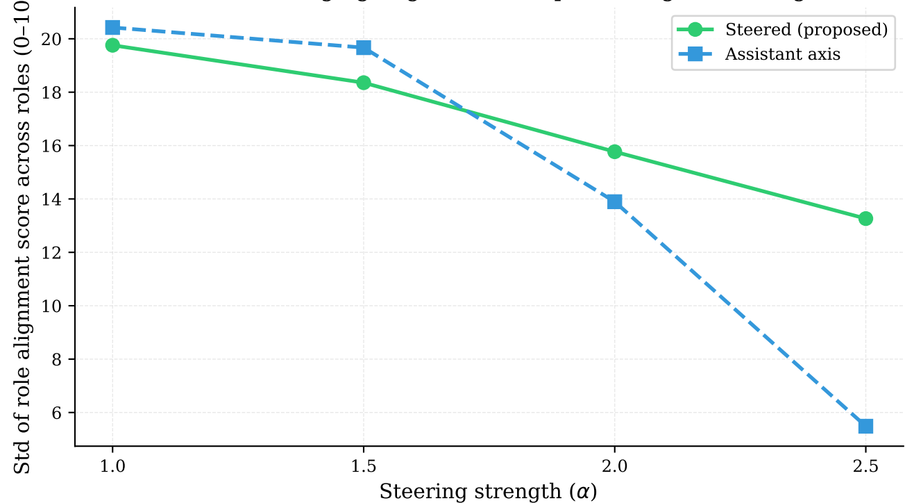
Inter-role score variance: std of role alignment scores across 275 roles (lower = roles converging; higher = roles preserving distinct signatures)
