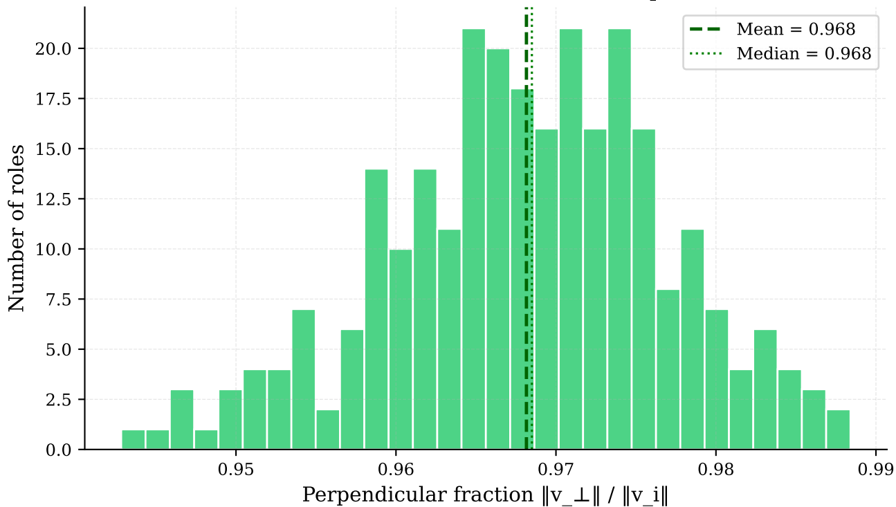
Role-specific fraction of each proposed vector (fraction the assistant axis cannot replicate)
