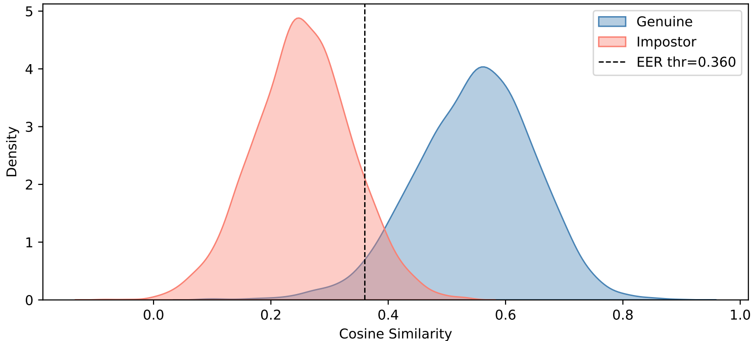
African — Gaussian Blur ( \sigma=0 )
