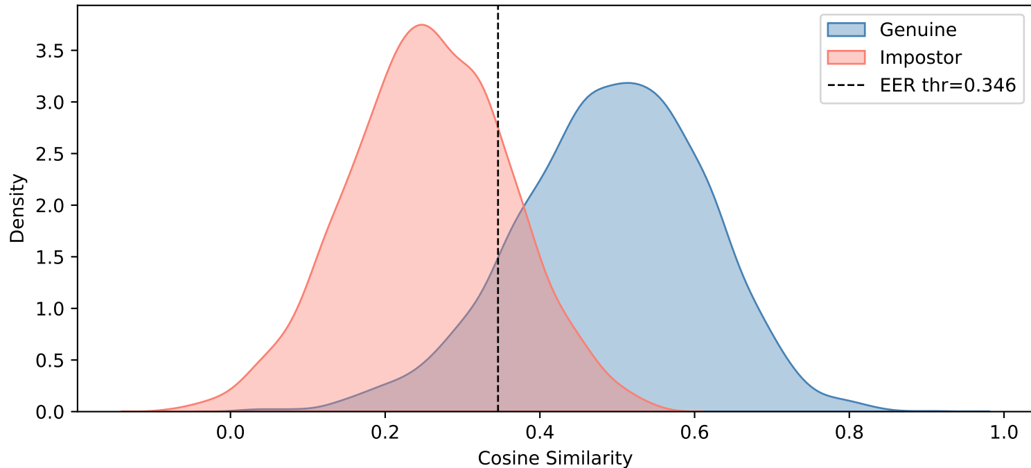
African — Gaussian Blur ( \sigma=2 )
