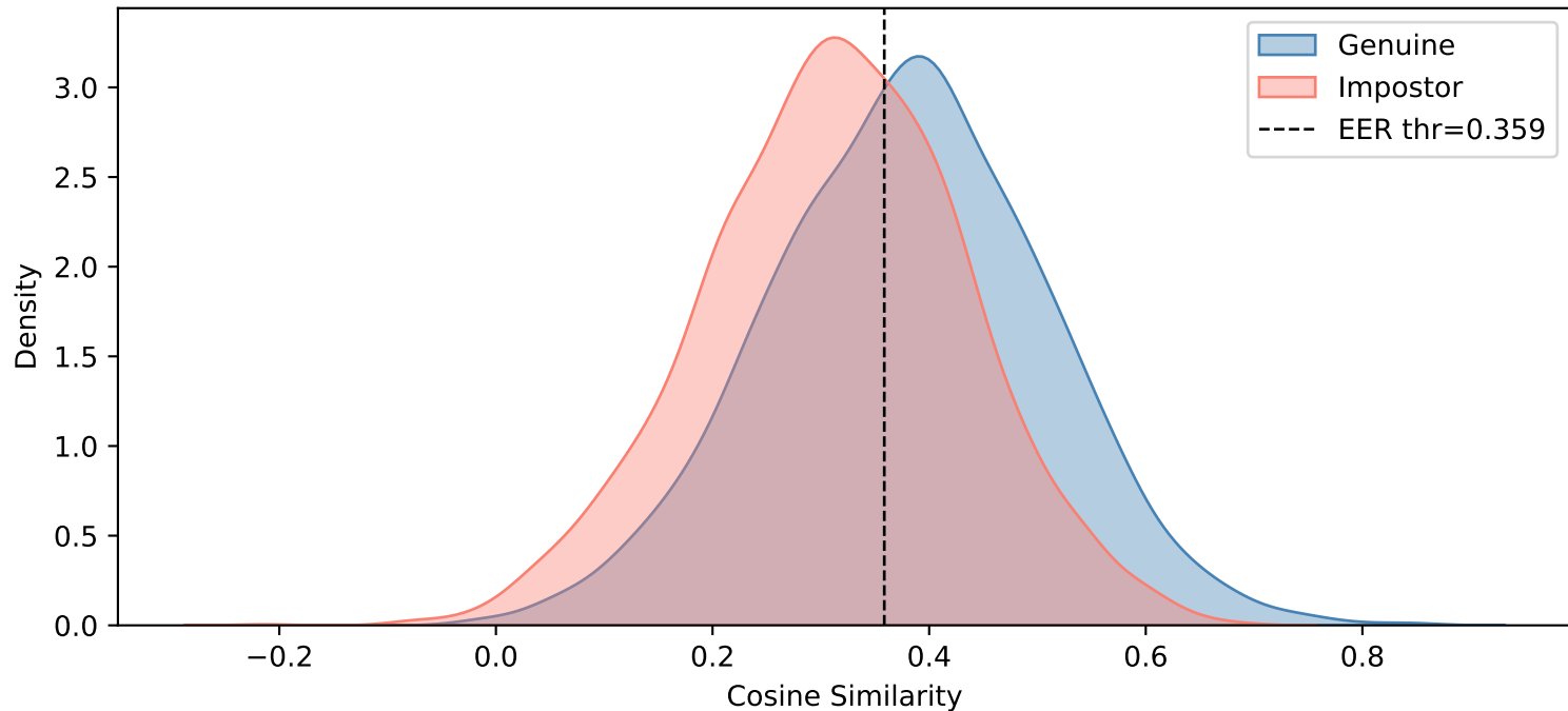
African — Motion Blur (k=21)
