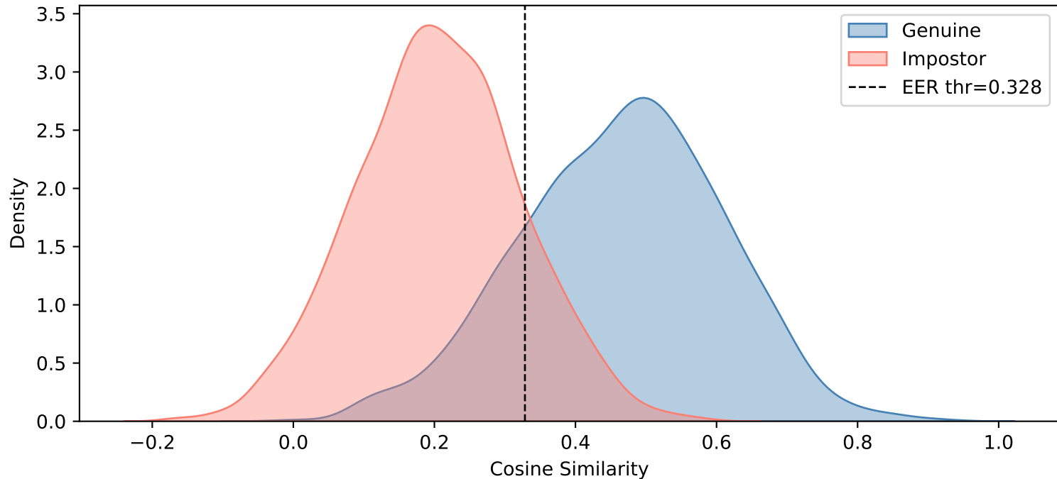
Asian — Gaussian Blur ( \sigma=2.4 )
