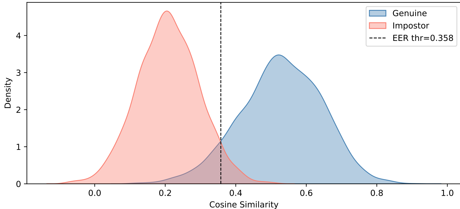
Asian — JPEG Compression (q=80)
