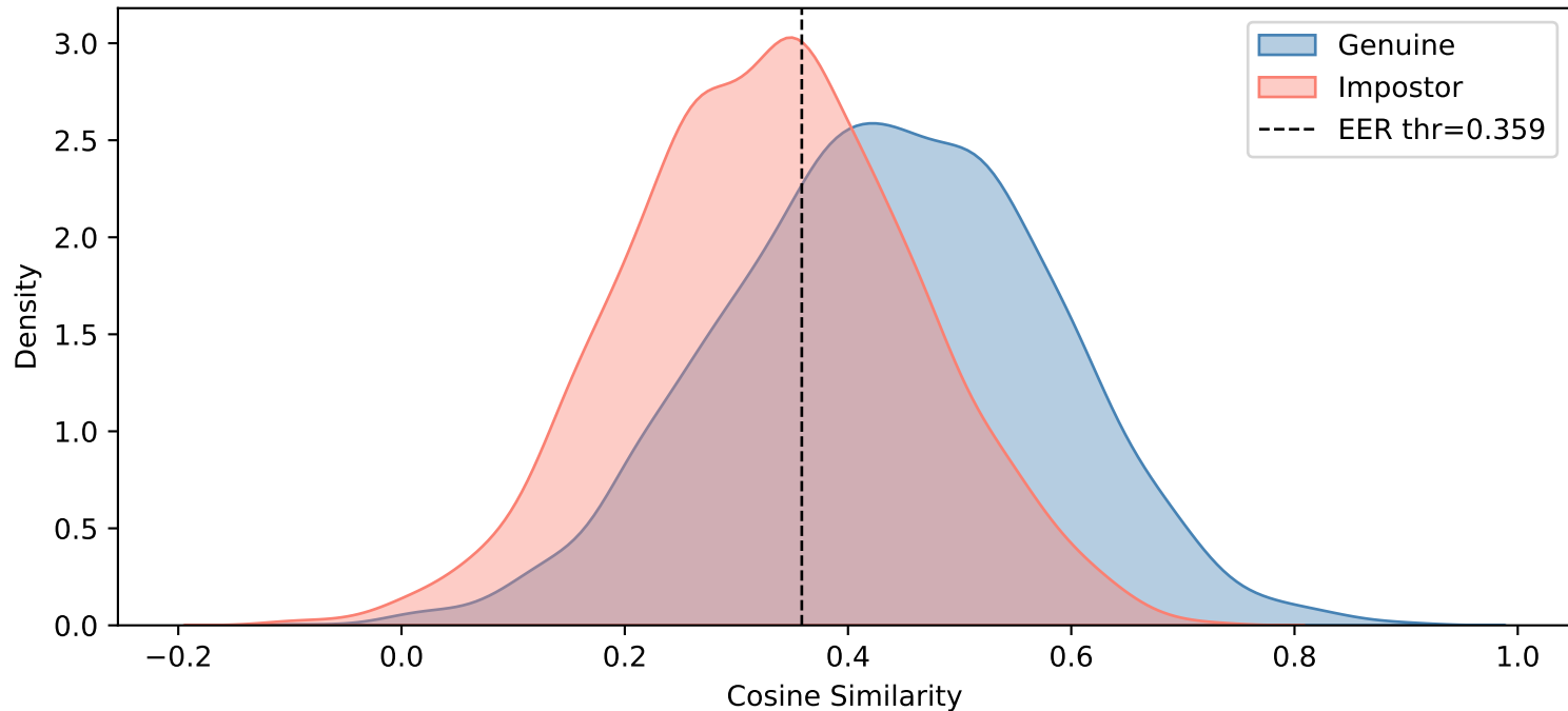
Asian — Motion Blur (k=21)
