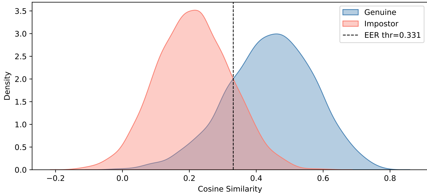
Caucasian — Salt & Pepper Noise ( p=0.06 )
