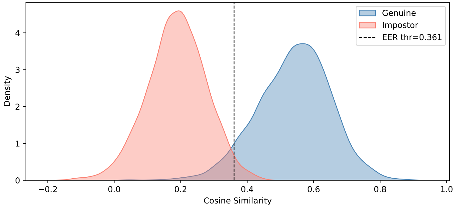
Caucasian — Brightness ( \beta=0.9 )
