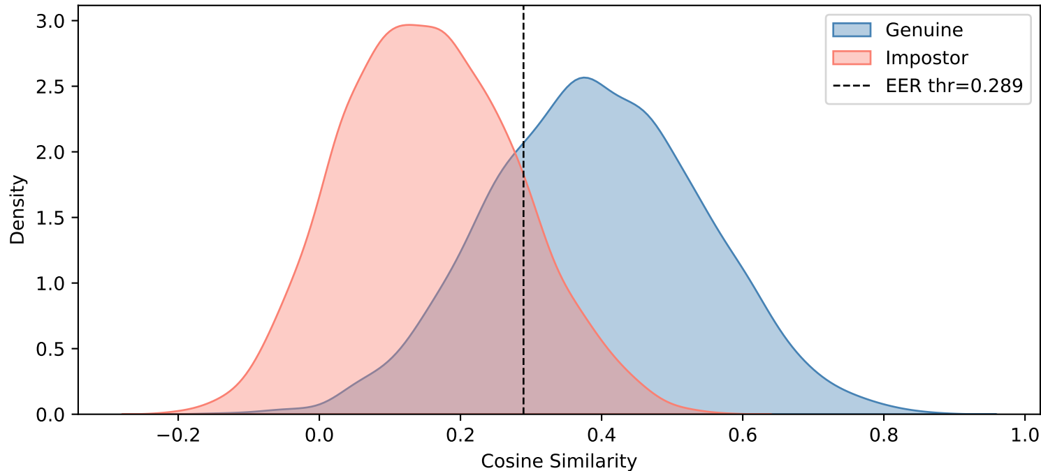
Caucasian — Gaussian Blur ( \sigma=3.2 )
