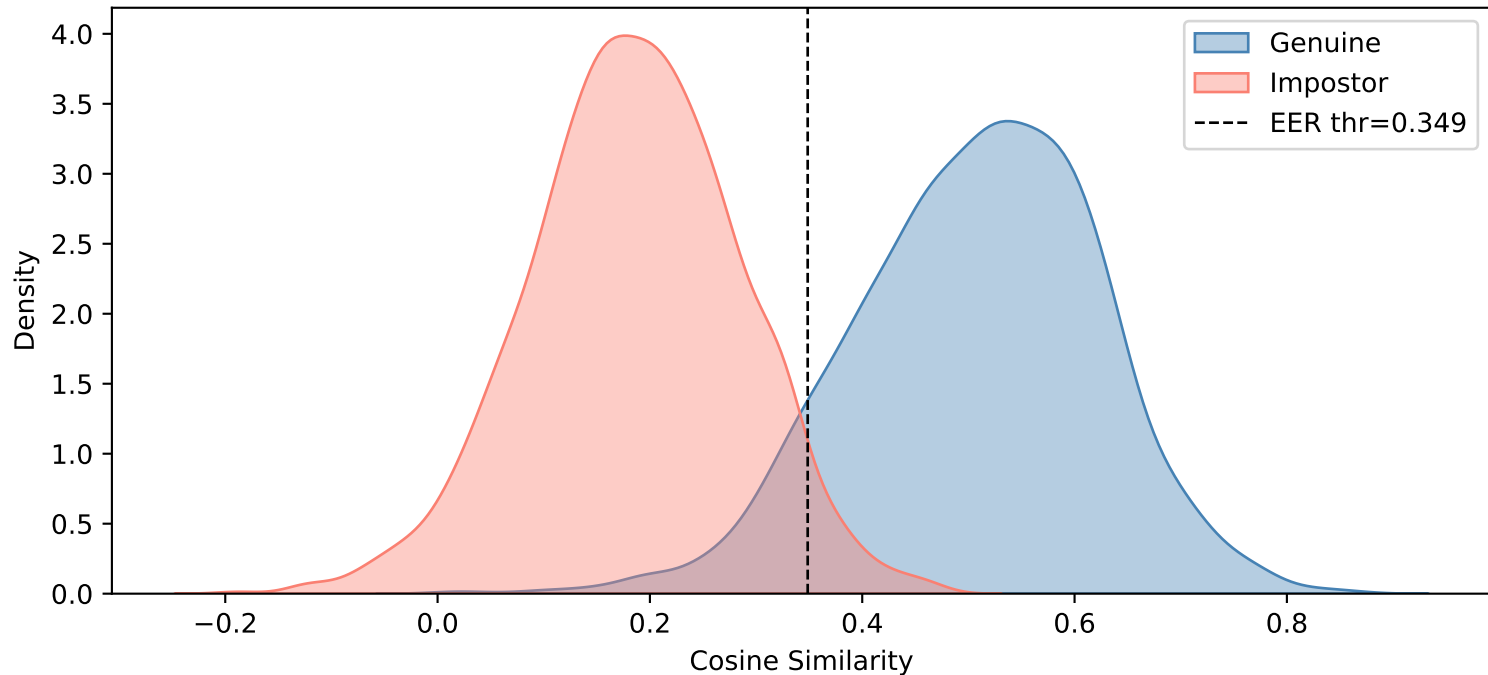
Caucasian — Gaussian Noise ( \sigma=8 )
