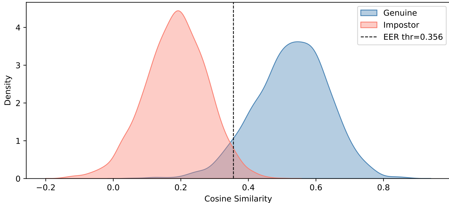
Caucasian — JPEG Compression (q=60)
