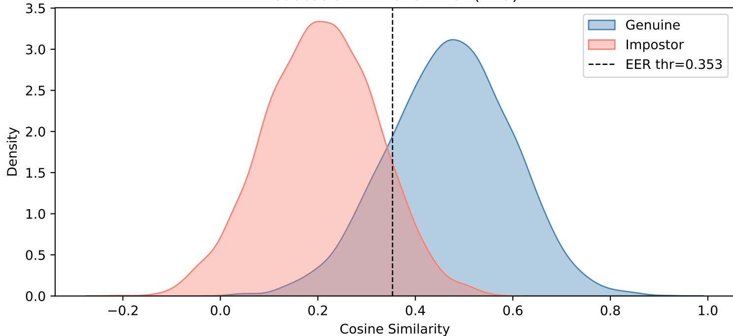
Caucasian — Motion Blur (k=9)
