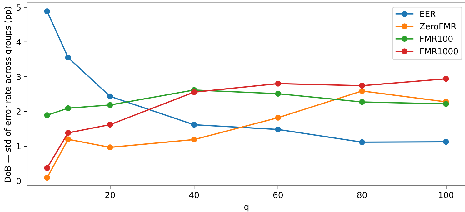
Degree of Bias — JPEG Compression
