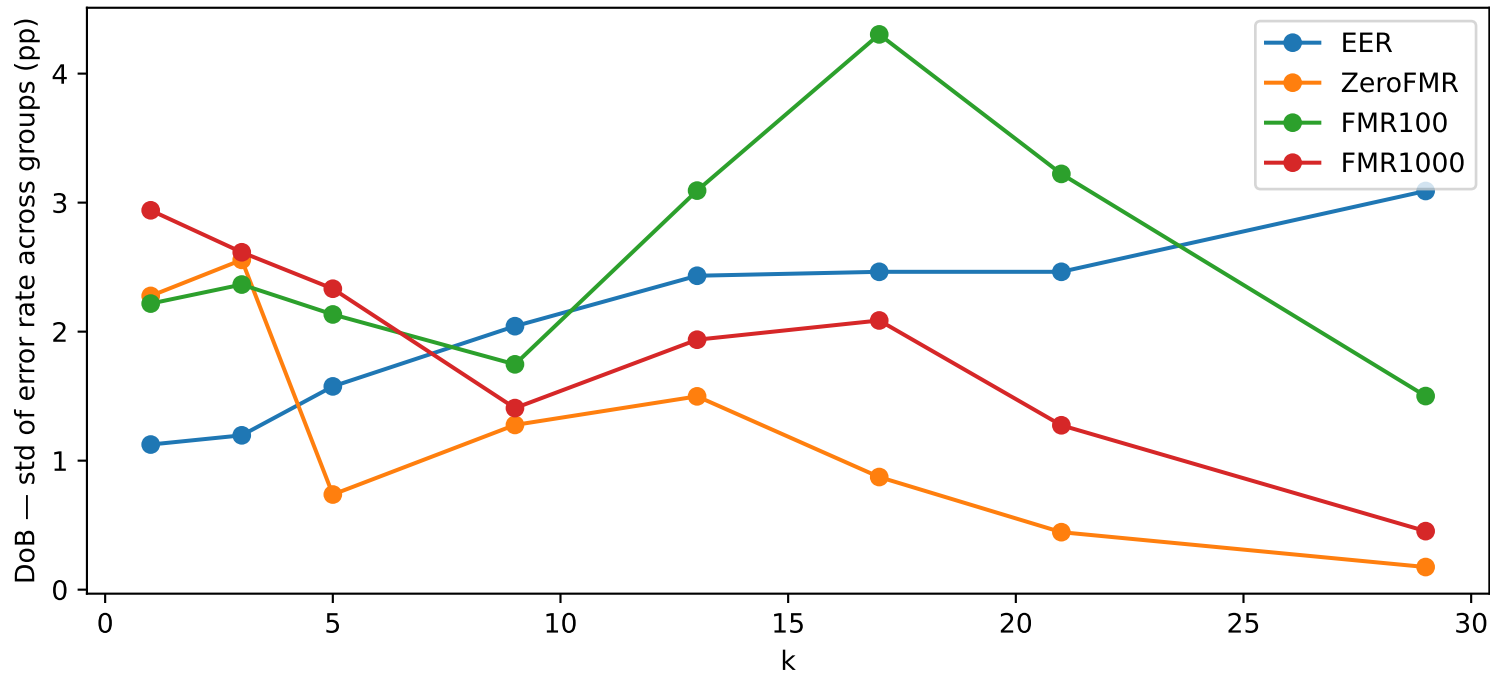
Degree of Bias — Motion Blur
