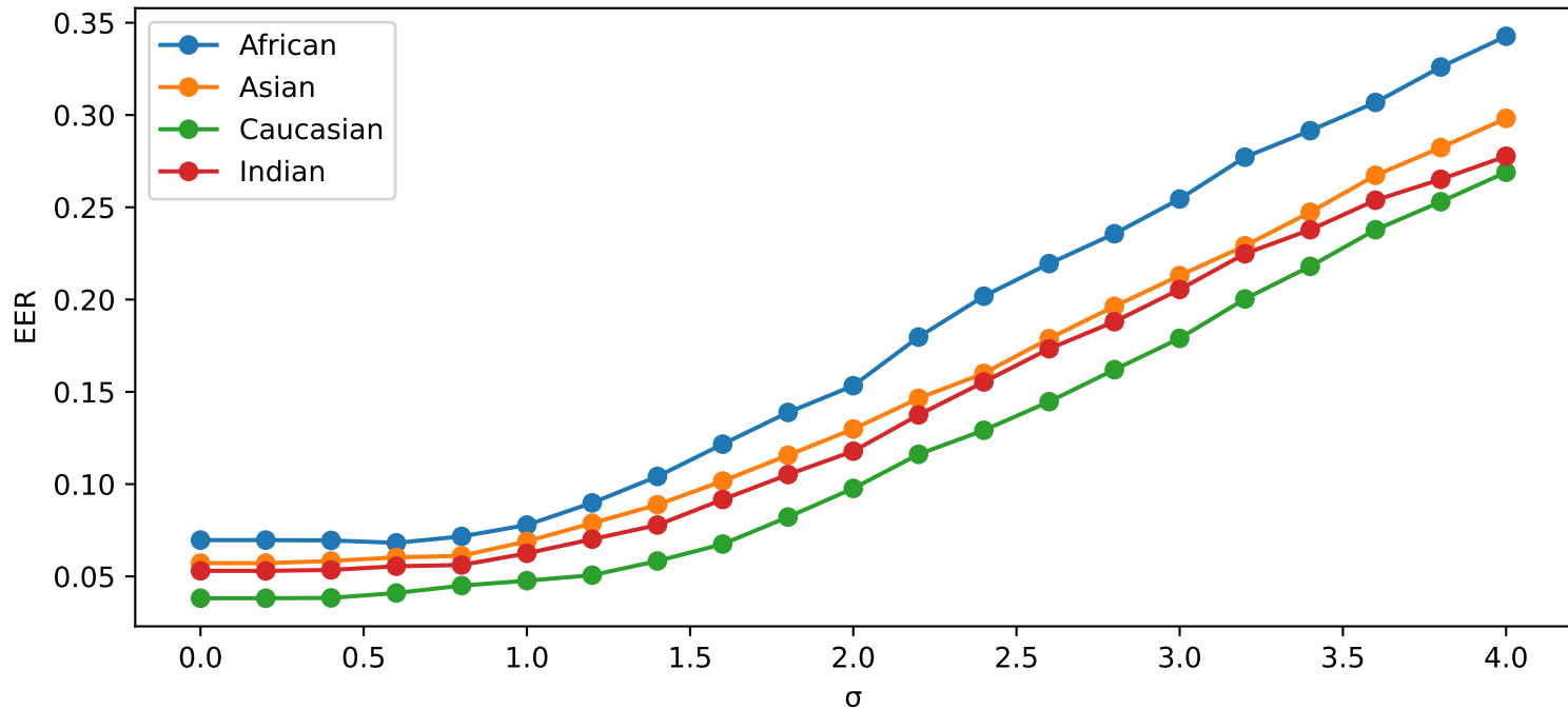
EER — Gaussian Blur
