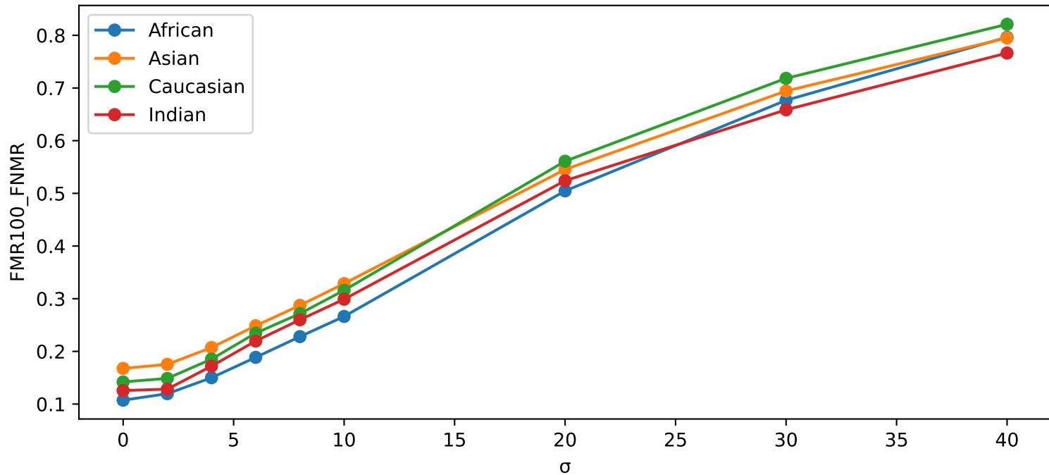
FMR100_FNMR — Gaussian Noise
