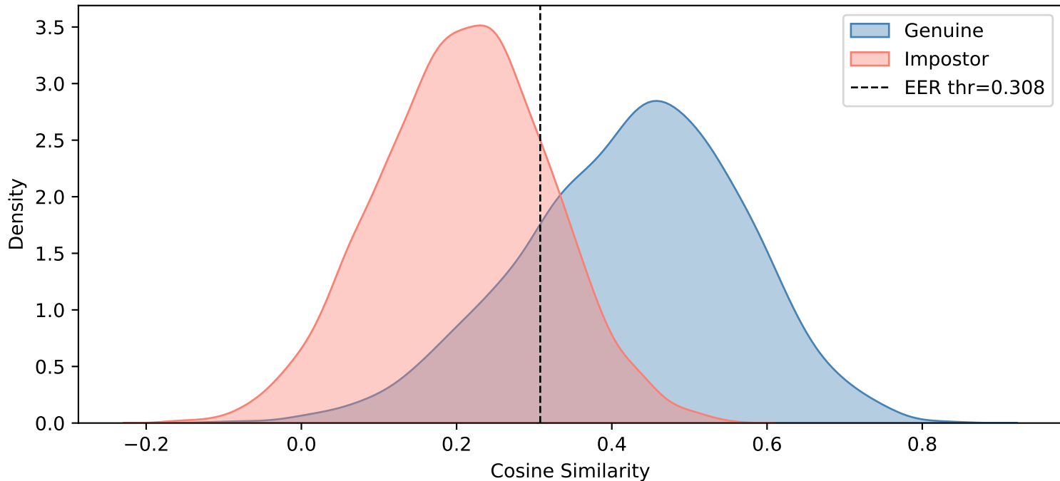
Indian — Contrast ( \alpha=4 )
