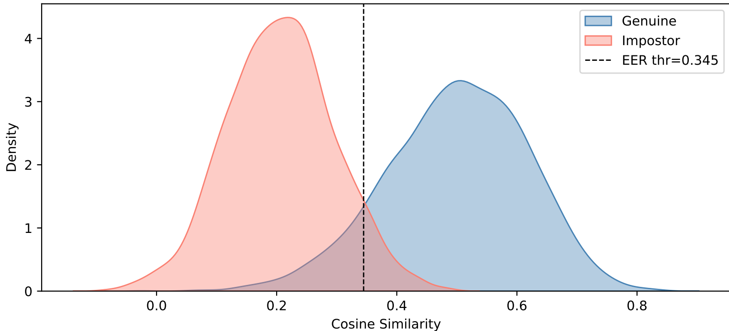
Indian — Gaussian Noise ( \sigma=10 )
