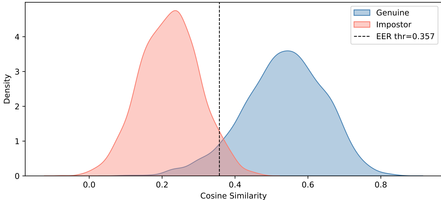
Indian — Gaussian Noise ( \sigma=4 )
