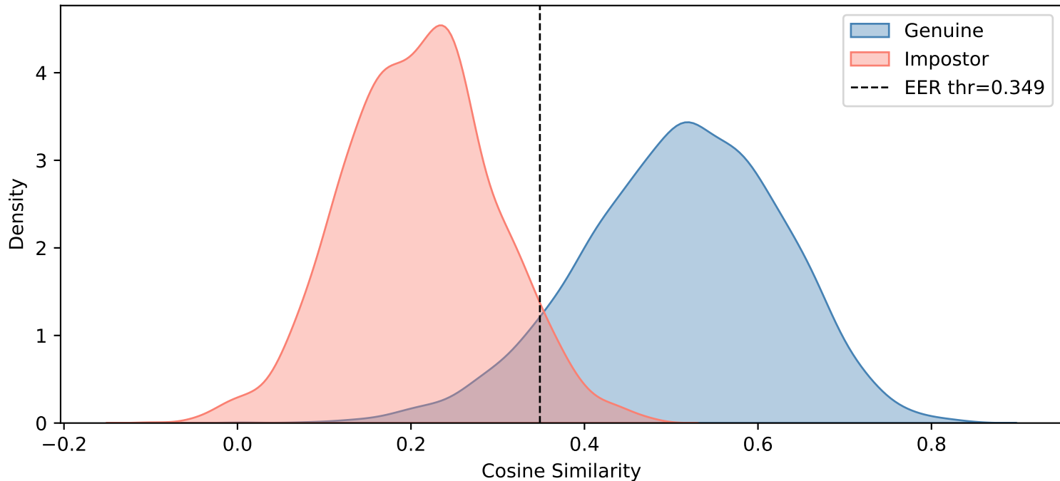
Indian — Gaussian Noise ( \sigma=8 )
