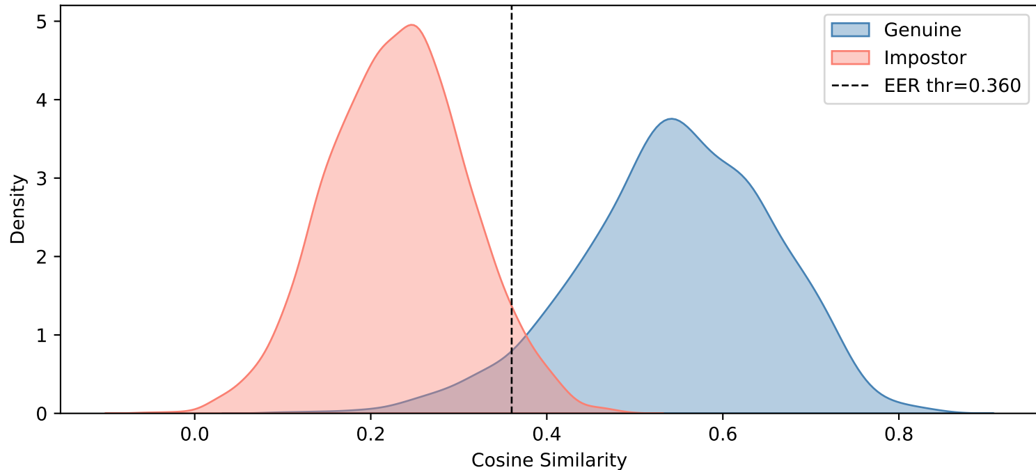
Indian — JPEG Compression (q=100)
