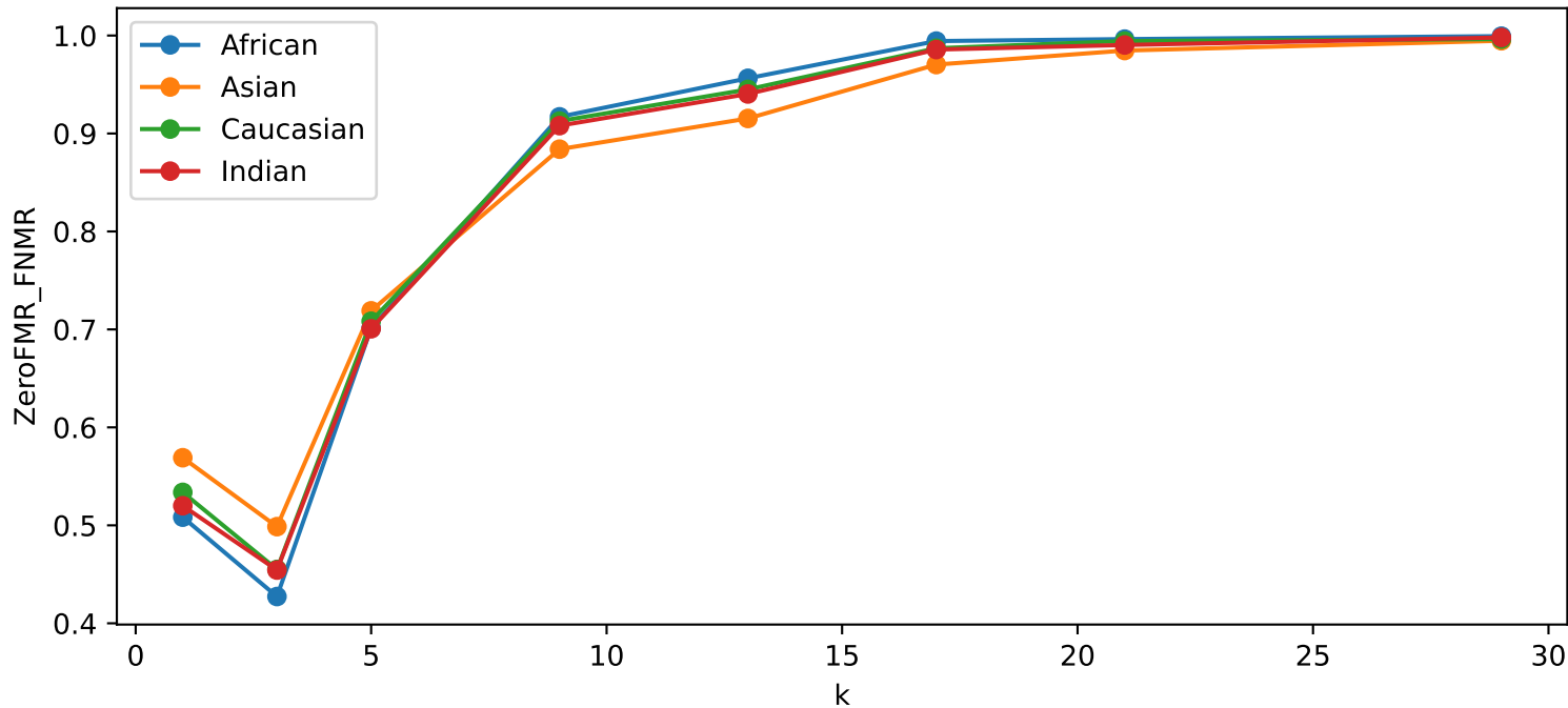
ZeroFMR_FNMR — Motion Blur
