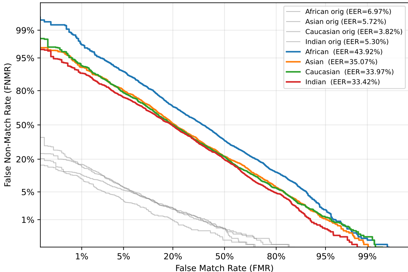
DET — Salt & Pepper Noise ( p=0.21 )
