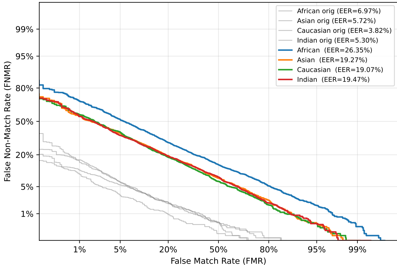
DET — Contrast ( \alpha=4 )
