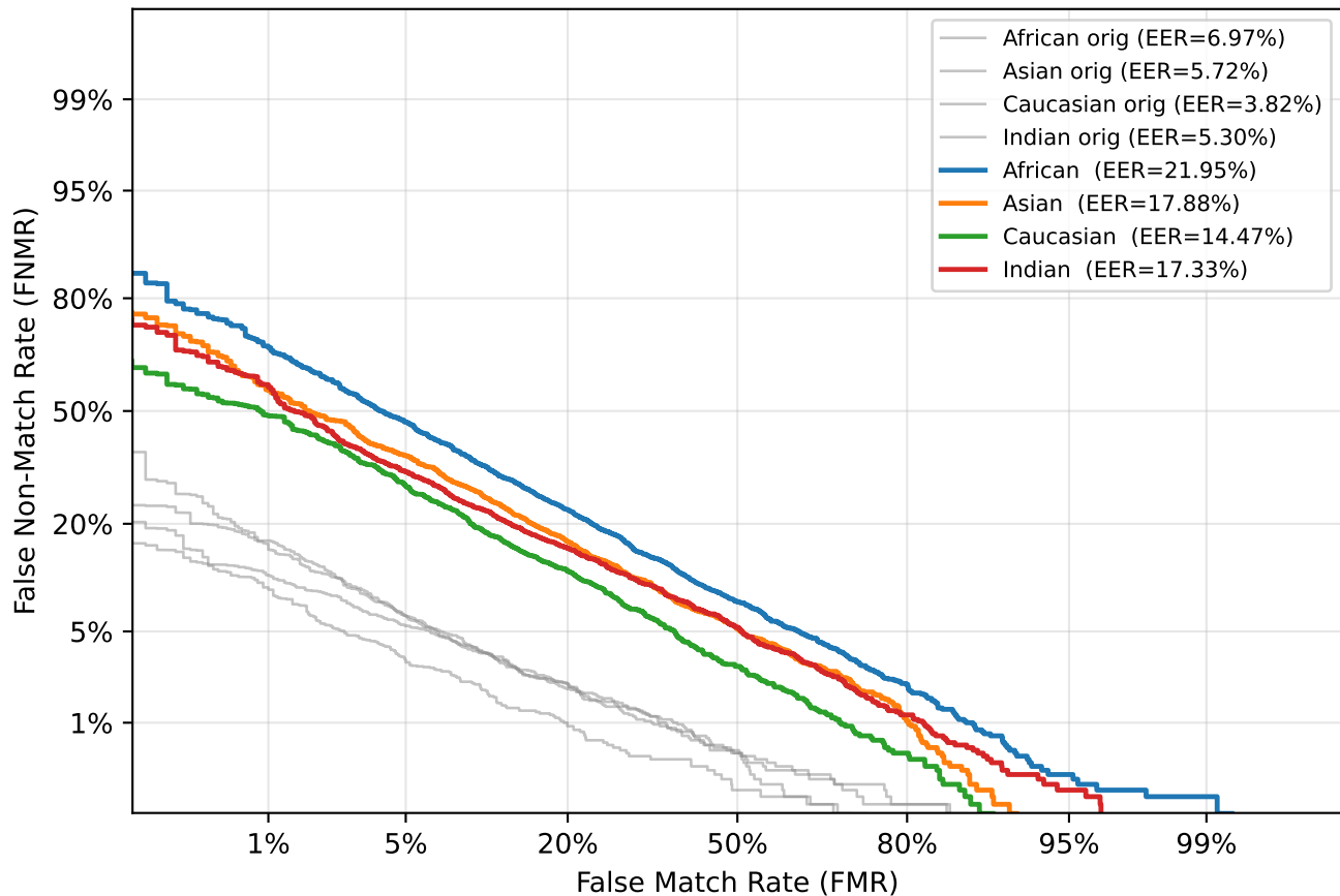
DET — Gaussian Blur ( \sigma=2.6 )
