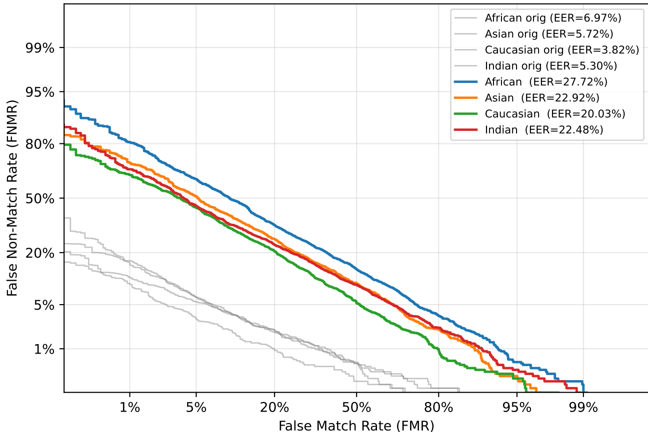
DET — Gaussian Blur ( \sigma=3.2 )
