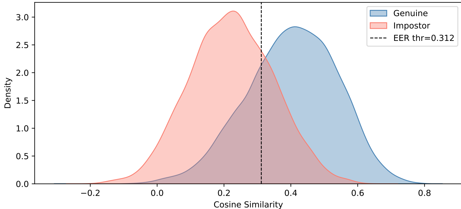
overall — Salt & Pepper Noise (p=0.09)
