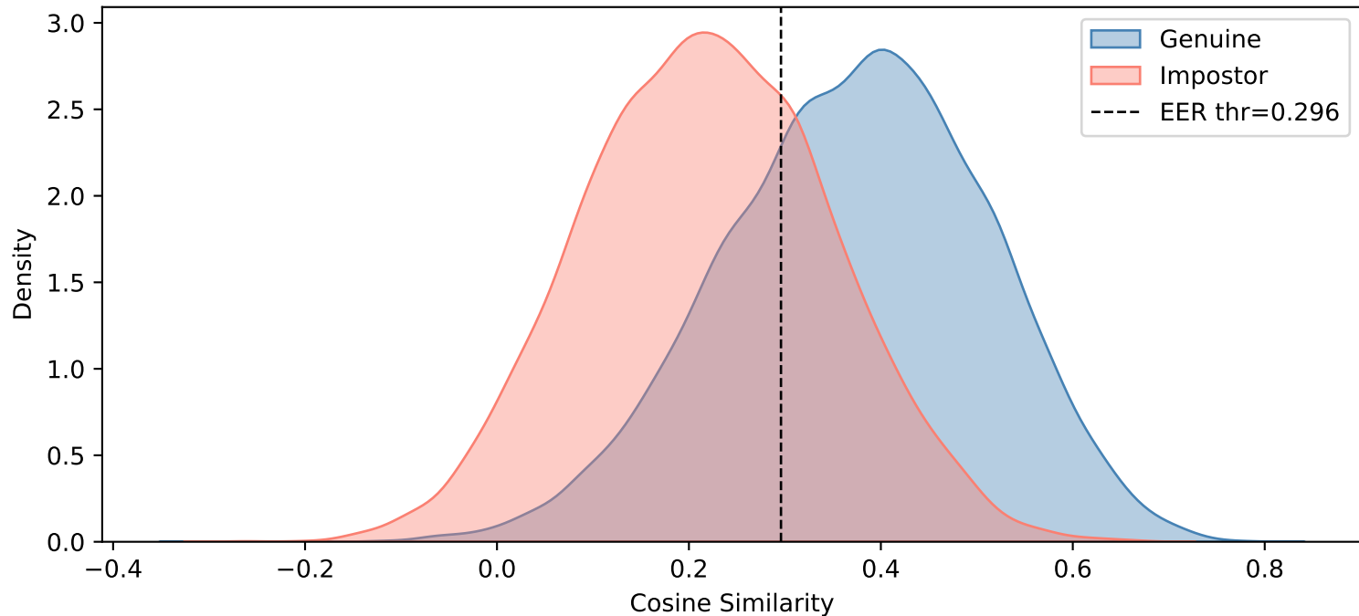
overall — Salt & Pepper Noise (p=0.12)
