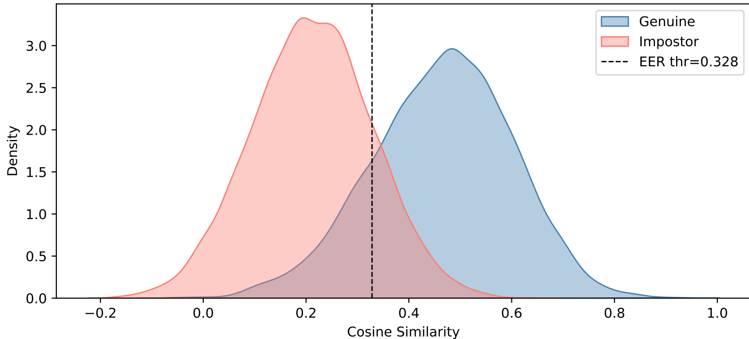
overall — Gaussian Blur ( \sigma=2.4 )
