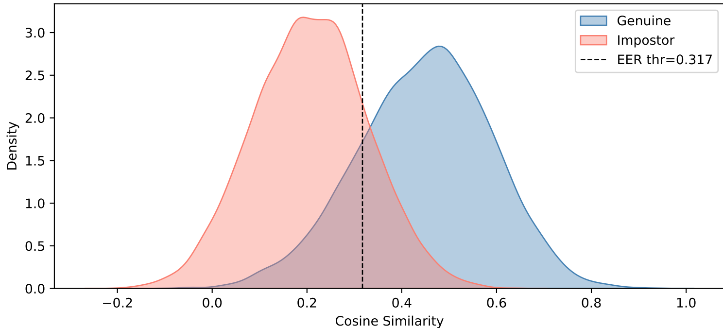
overall — Gaussian Blur ( \sigma=2.6 )
