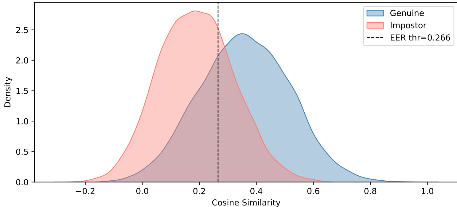
overall — Gaussian Blur ( \sigma=3.8 )
