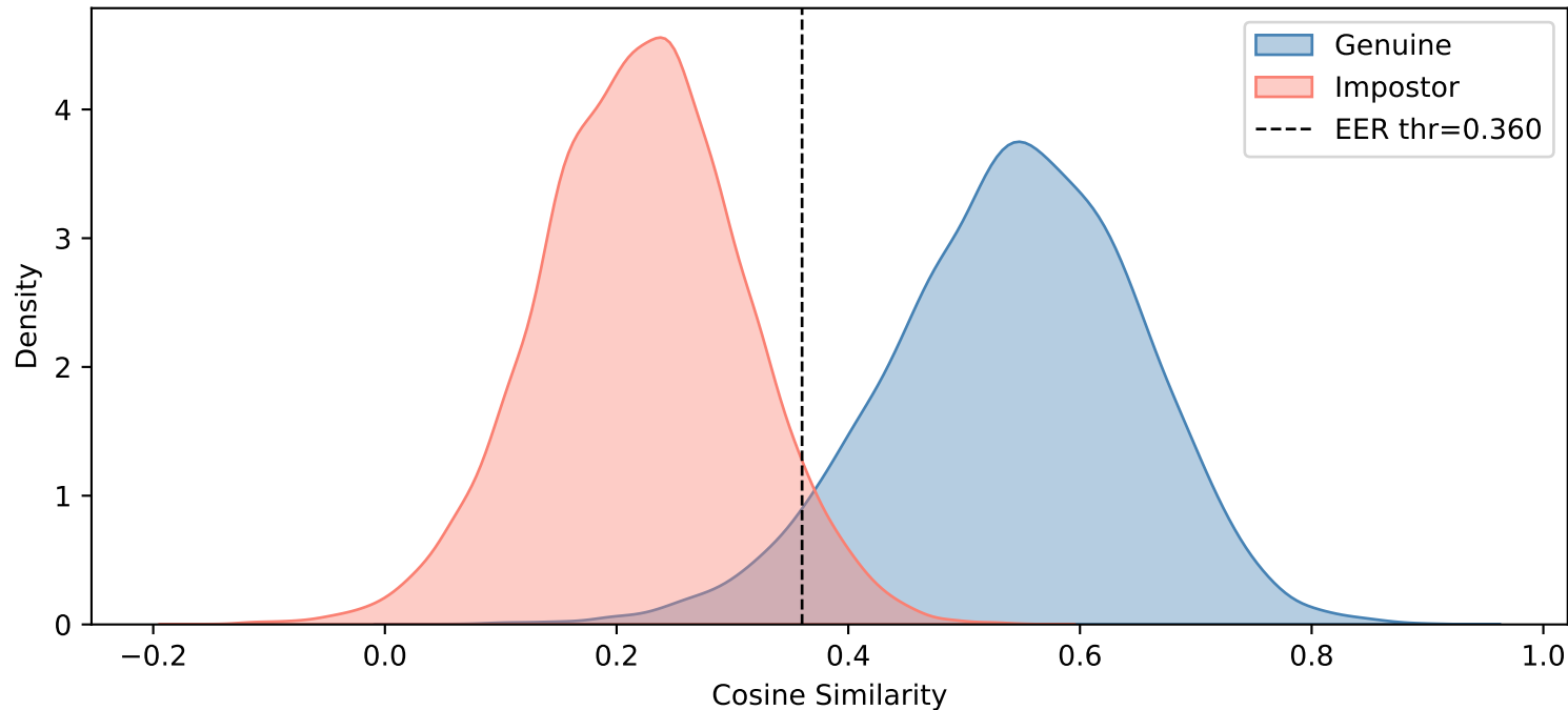
overall — Gaussian Noise ( \sigma=0 )
