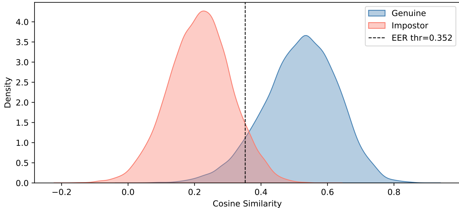
overall — JPEG Compression (q=40)
