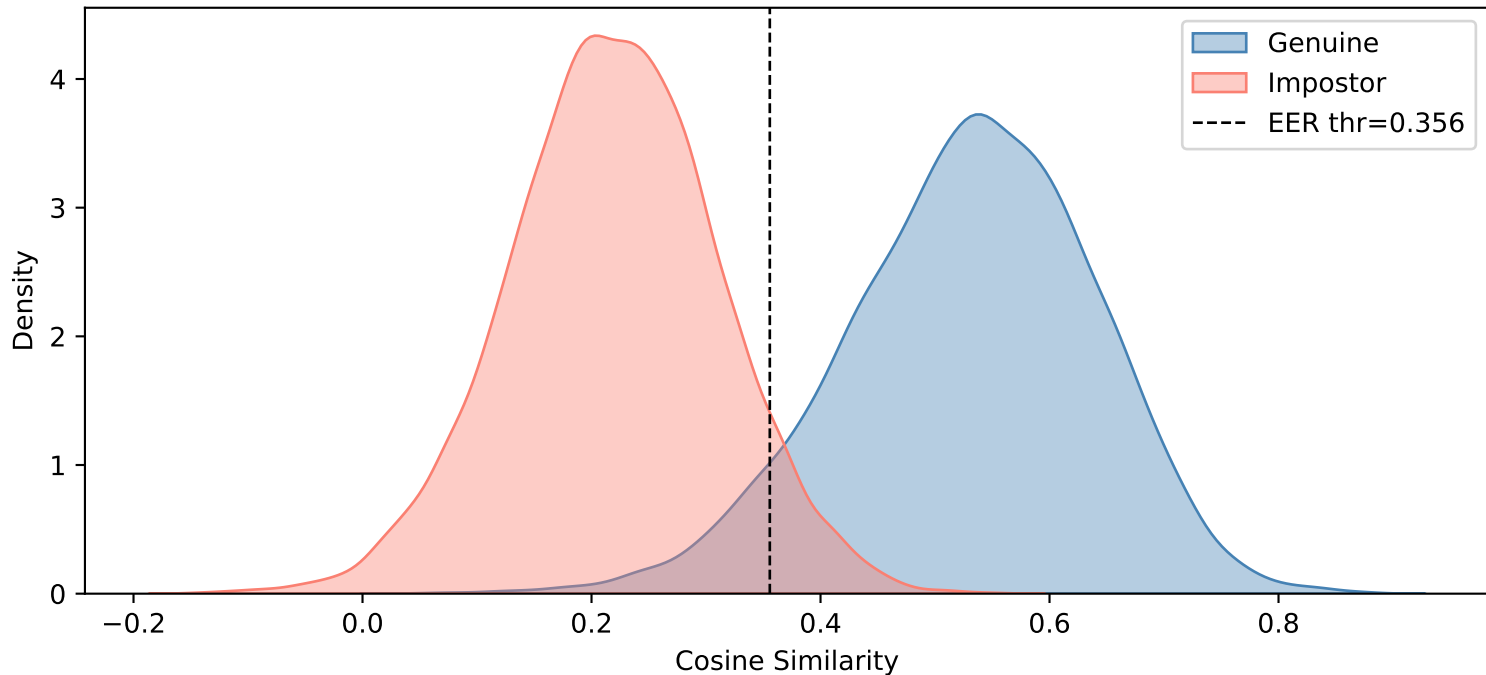
overall — JPEG Compression (q=60)
