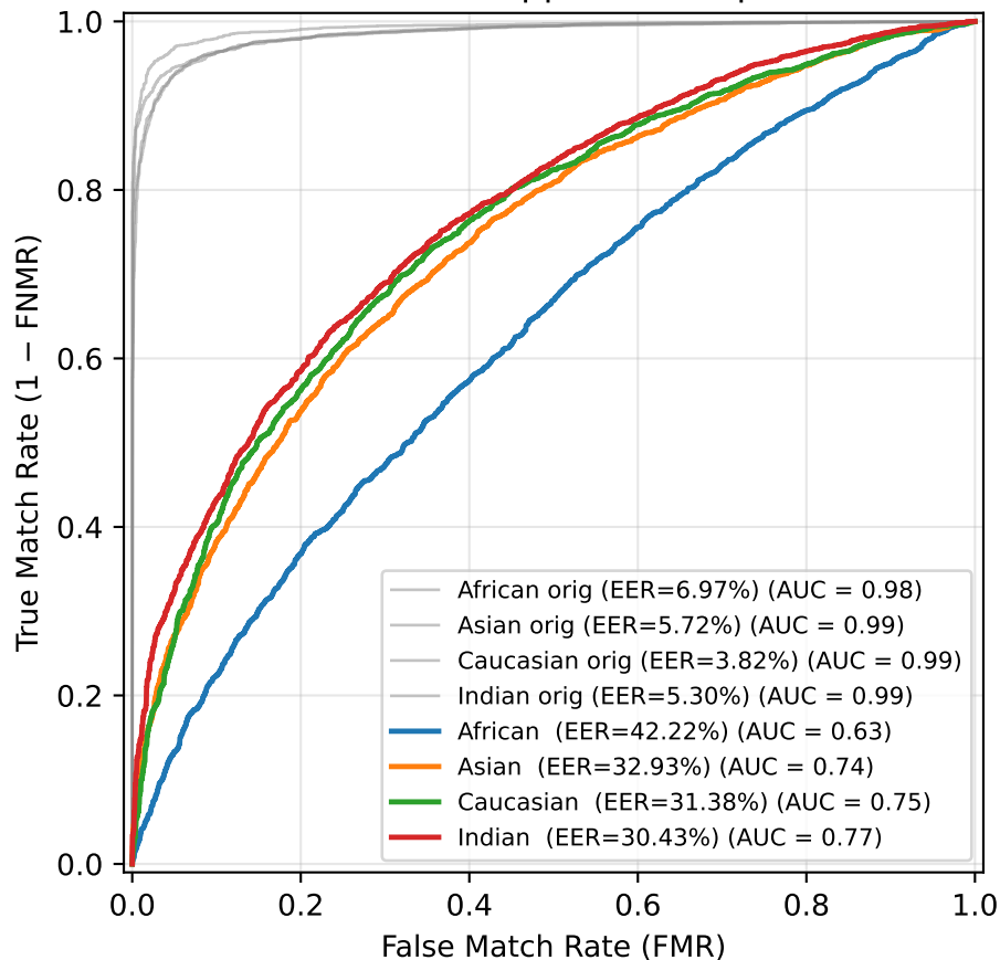
ROC — Salt & Pepper Noise ( p=0.18 )
