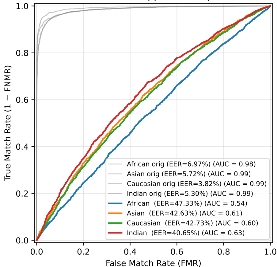
ROC — Salt & Pepper Noise (p=0.3)
